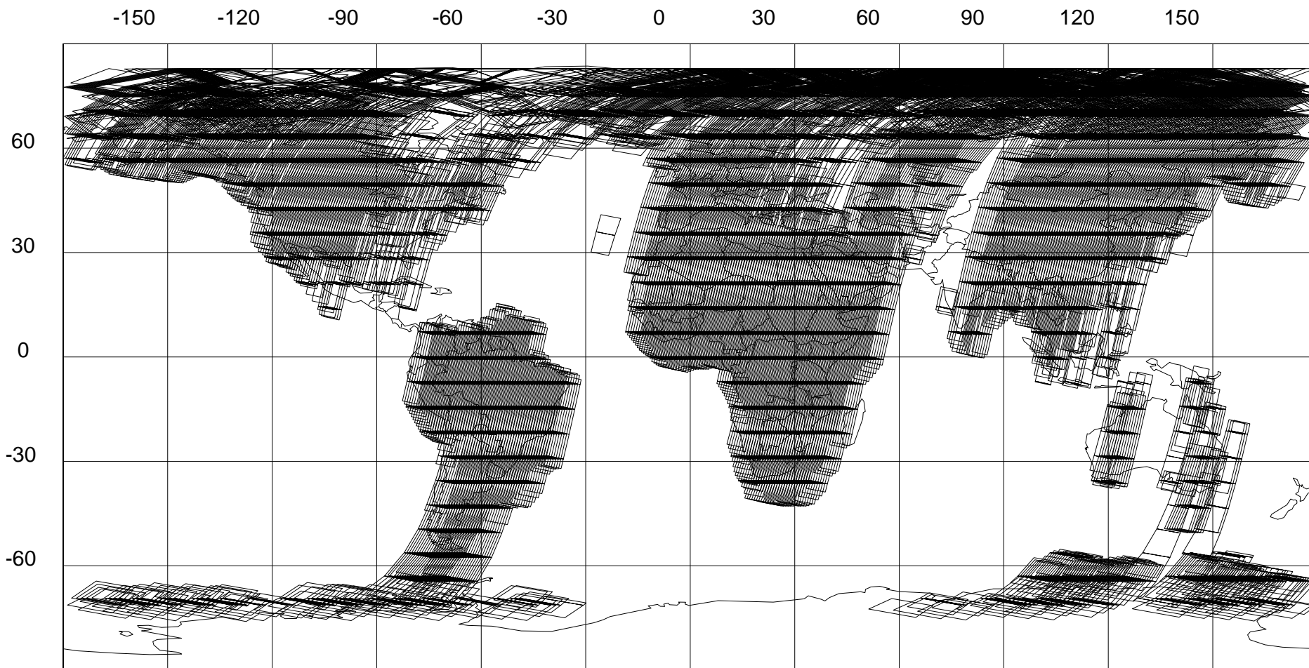
ATSR-2 High Rate Coverage Cycle 14 12 August through 16 September 1996.
