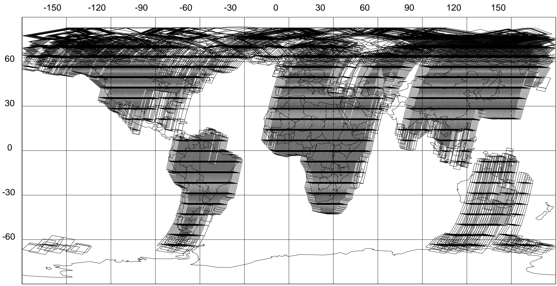
ATSR-2 High Rate Coverage Cycle 24 28th July through 01 Sept. 1997 ESA/ESTEC/NW, ERS-2, 35-day repeat orbit ( 501), -71.723 deg First Orbit 11879 Last Orbit 12379
