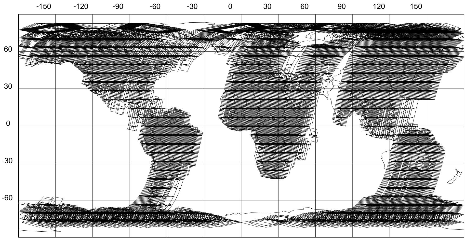
ATSR-2 High Rate Coverage Cycle 25 01 Sept. through 06 Oct. 1997 ESA/ESTEC/NW, ERS-2, 35-day repeat orbit ( 501), -71.723 deg First Orbit 12380 Last Orbit 12880
